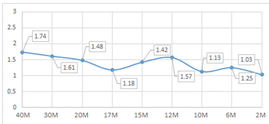
144 MHz – 7.0 MHz Dipole Analysis
