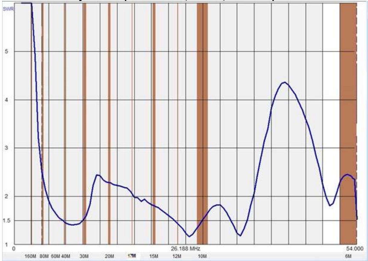
SWR Analysis on Tripod with NVIS, Vertical, & Counterpoise elements
