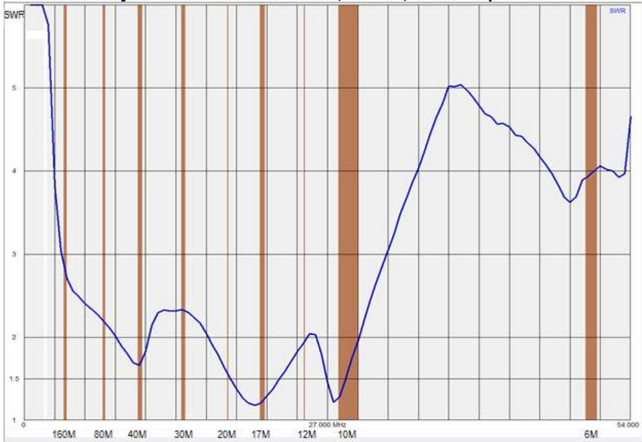
SWR Analysis on Jaw Mount with NVIS, Vertical, & Counterpoise elements
