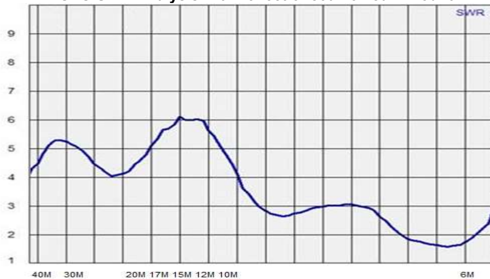
MOTO SWR Analysis with 25 feet of coax on Jam Mount
