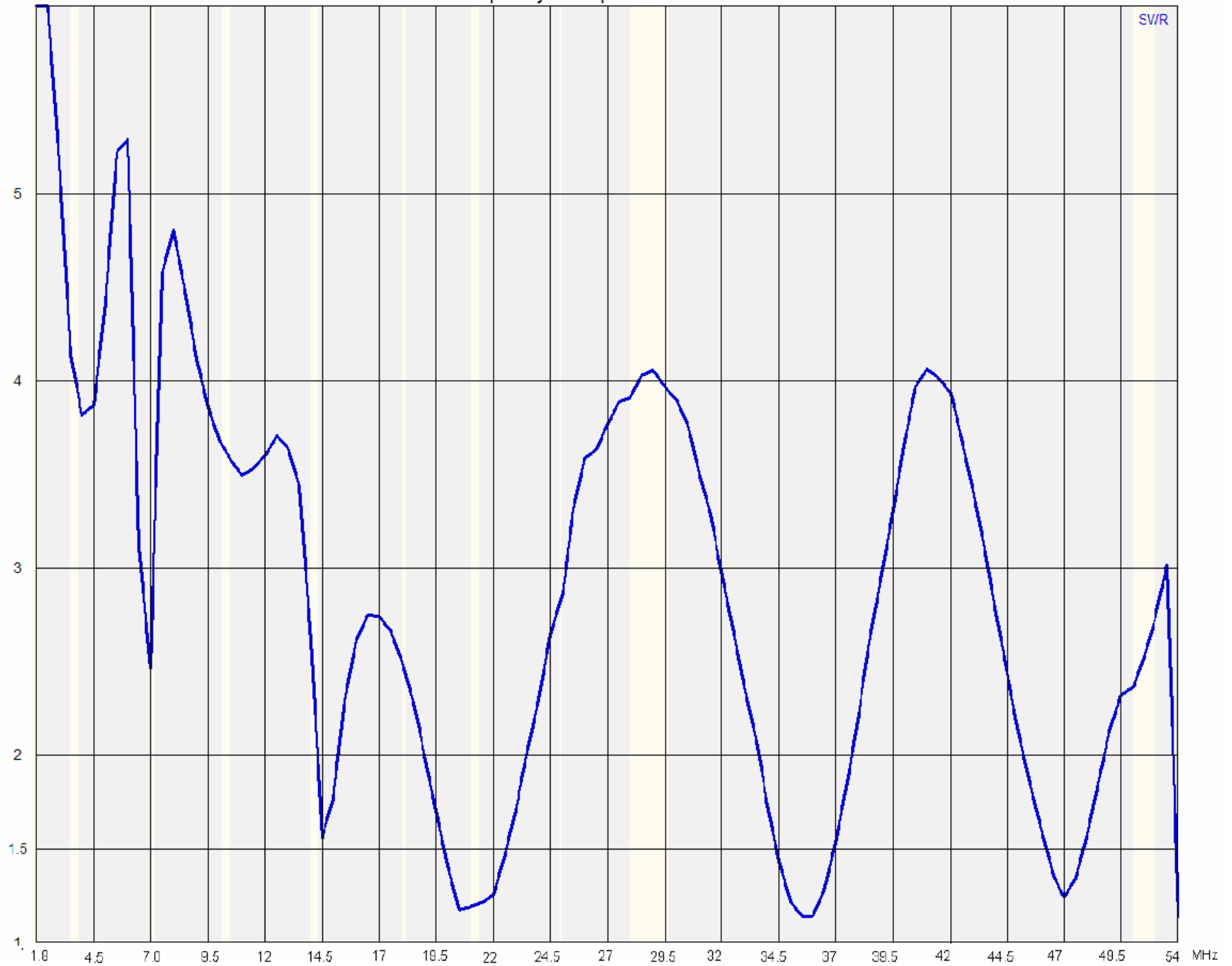
Rig Expert AA-54 Analysis of Alpha J-Pole Sr Antenna Antenna at a height of 6 ½ feet at coax feed point sloping upward to 13 feet at far end Fed with RG-58 Coax Frequency Sweep from 1.8-54MHz
