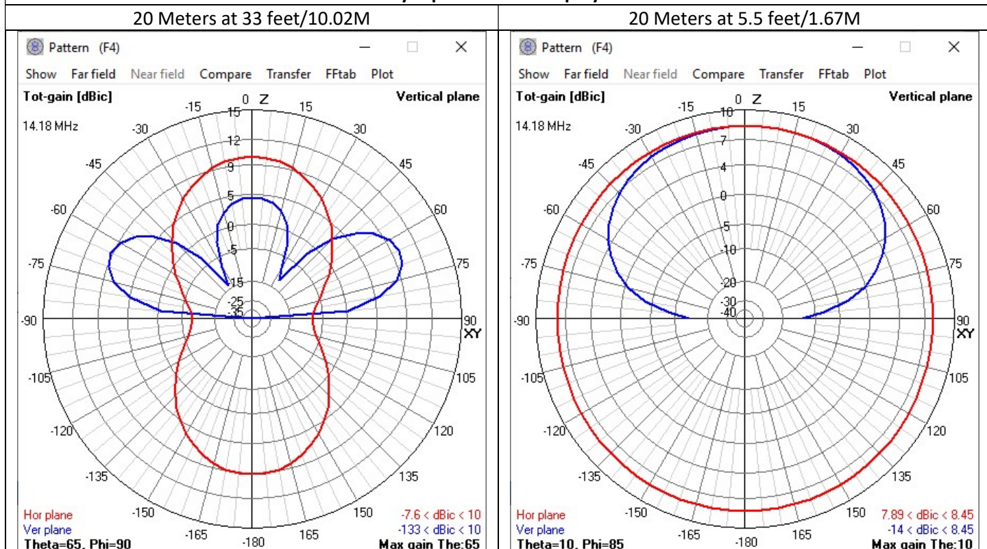
Gain of the HexTenna by Alpha Antenna deployed at 33 feet vs 5.5 feet
